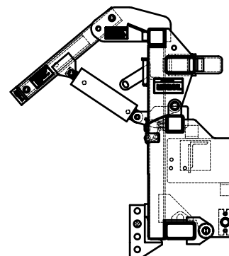
POWER TILT HD WING PIN HITCH Truck Portion
