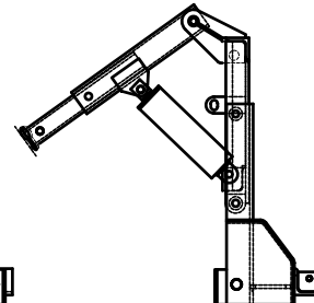
MANUAL TILT QUICK HITCH Truck Portion 30.5" and 33.5"
