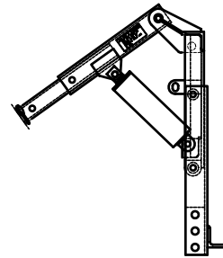
MANUAL TILT PIN HITCH Truck Portion 30.5" - 33.5" - 21"/30.5" COMBO
