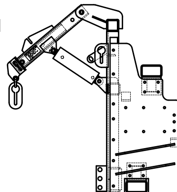
NON-TILT HD WING PIN HITCH Truck Portion
